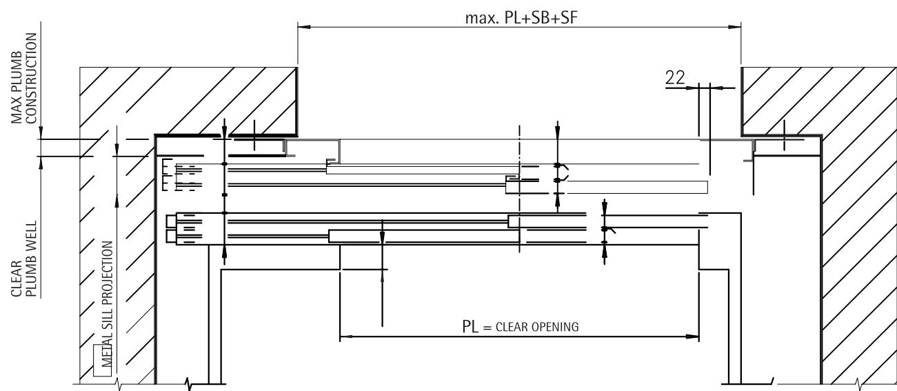
NICHE INSTALLATION
